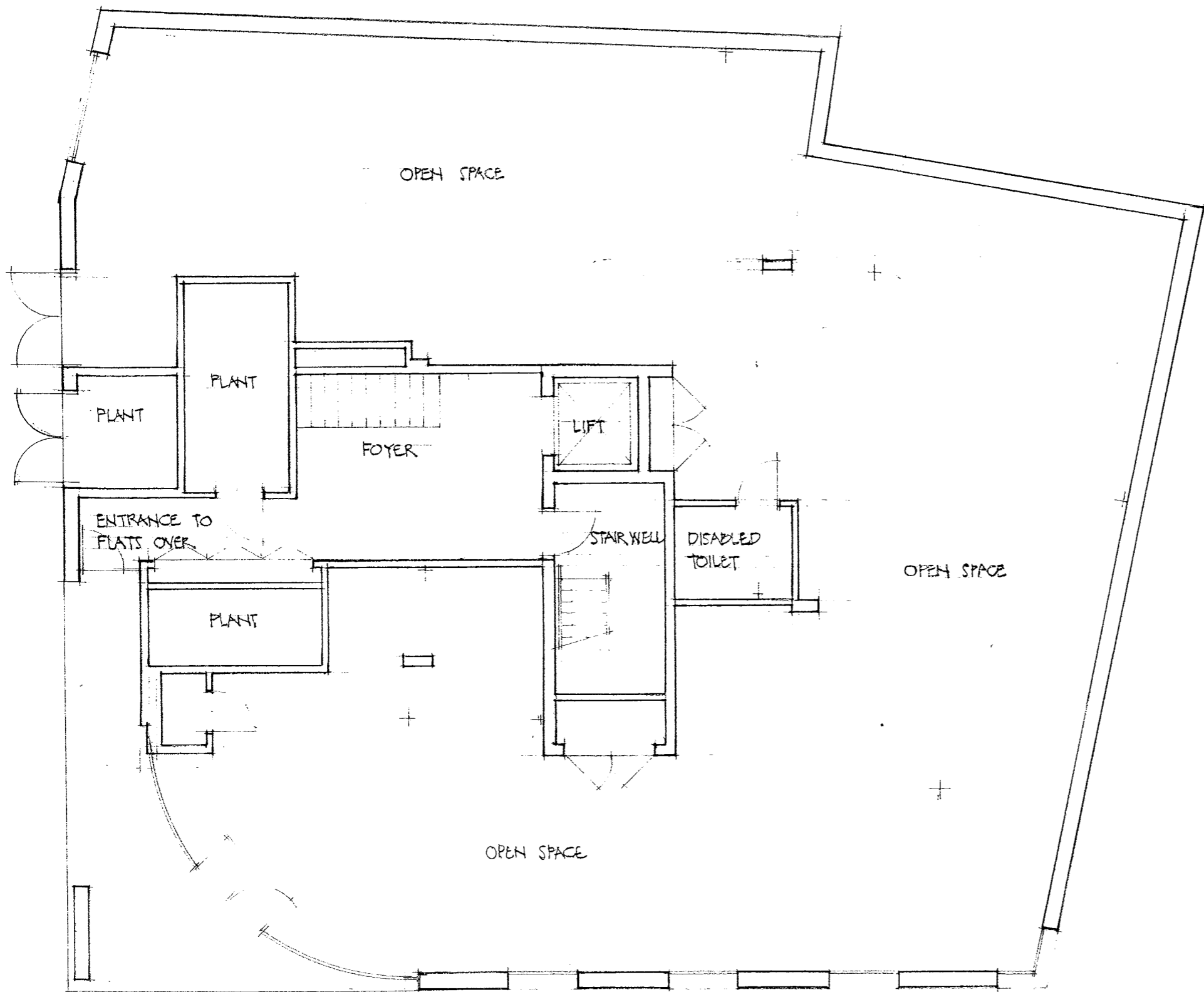
GROUND FLOOR PLAN EXISTING LAYOUT
